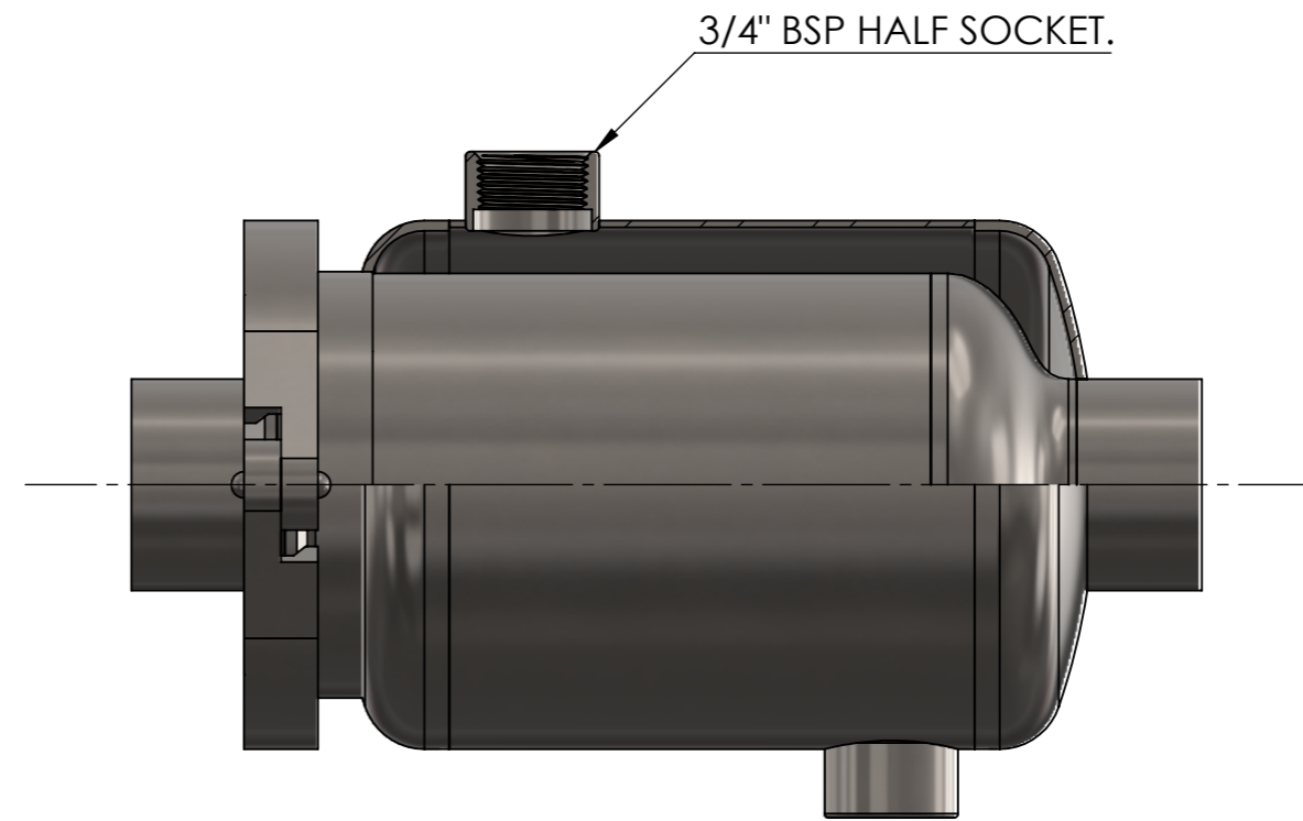
SECTION C-C
