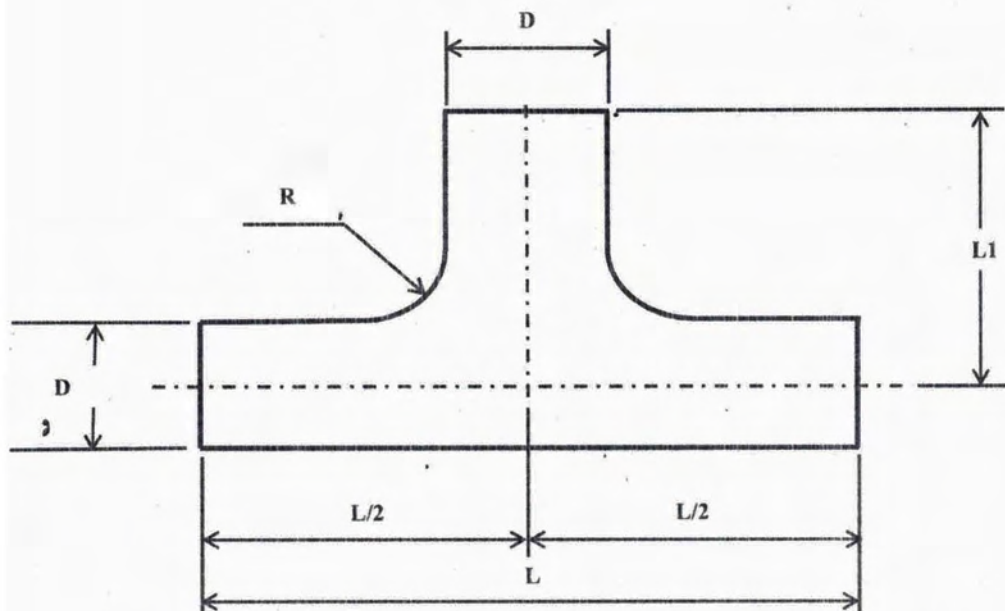
FIGURE C-SIZE DESIGNATION FOR EQUAL RADIUS TEES
